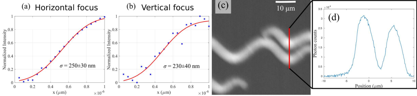
Fig. 2. SCXM scanning results. Focus scan results for the (a) horizontal and (b) vertical focus. The normalized Compton signal is represented by the blue crosses. The red line represents the best fit to an error function. The estimated \sigma for each error function is displayed. (c) Spirulina SCXM image at 60 keV with 100 nm steps and 100 ms dwell time. The scale bar corresponds to 10 \mu\text{m} . (d) Line profile over the red line. The background contrast has been subtracted.
